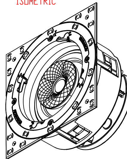
ISOMETRIC
