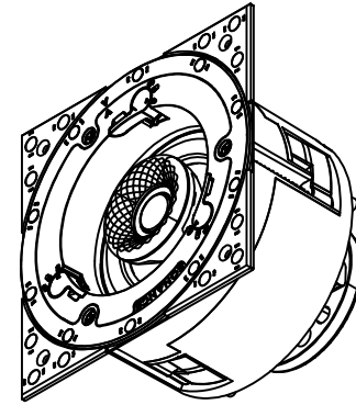
ISOMETRIC
