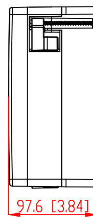
MOUNTING DEPTH
